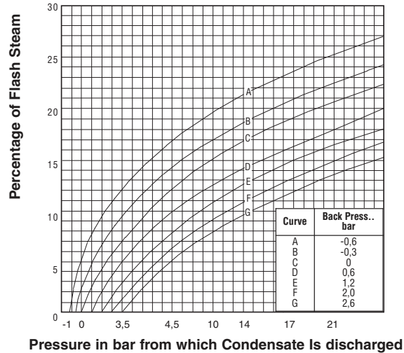
Percentage of Flash Steam formed when discharging Condensate to Reduced Pressure
